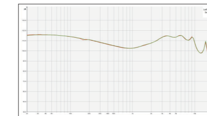
*Left & Right Sensitivity Curve: (50-100: ±5dB; 101-3K: ±3dB; 3.001K-5K: ±6dB; 5.001K-10K: ±8dB; 1K&R: ±3dB)
